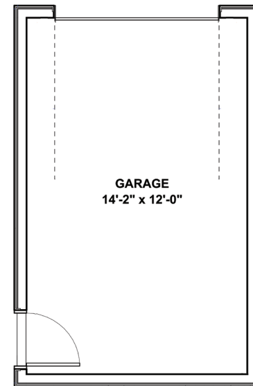
Detached Garage Side entry door location is plan-specific
