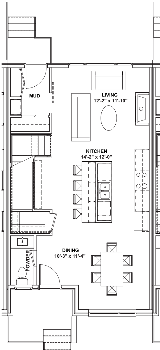
First Floor
