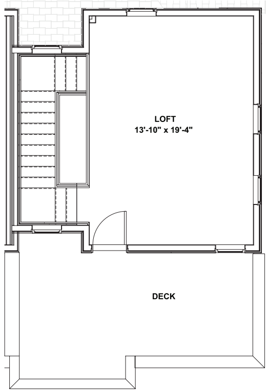
Third Floor
