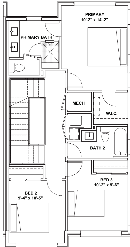
Second Floor
